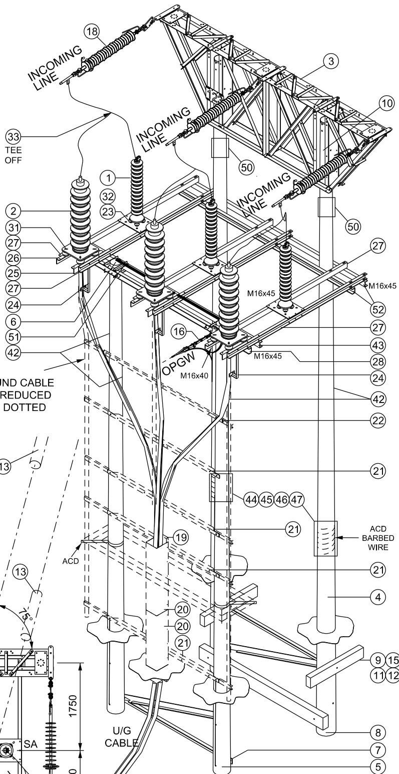
ISOMETRIC VIEW
