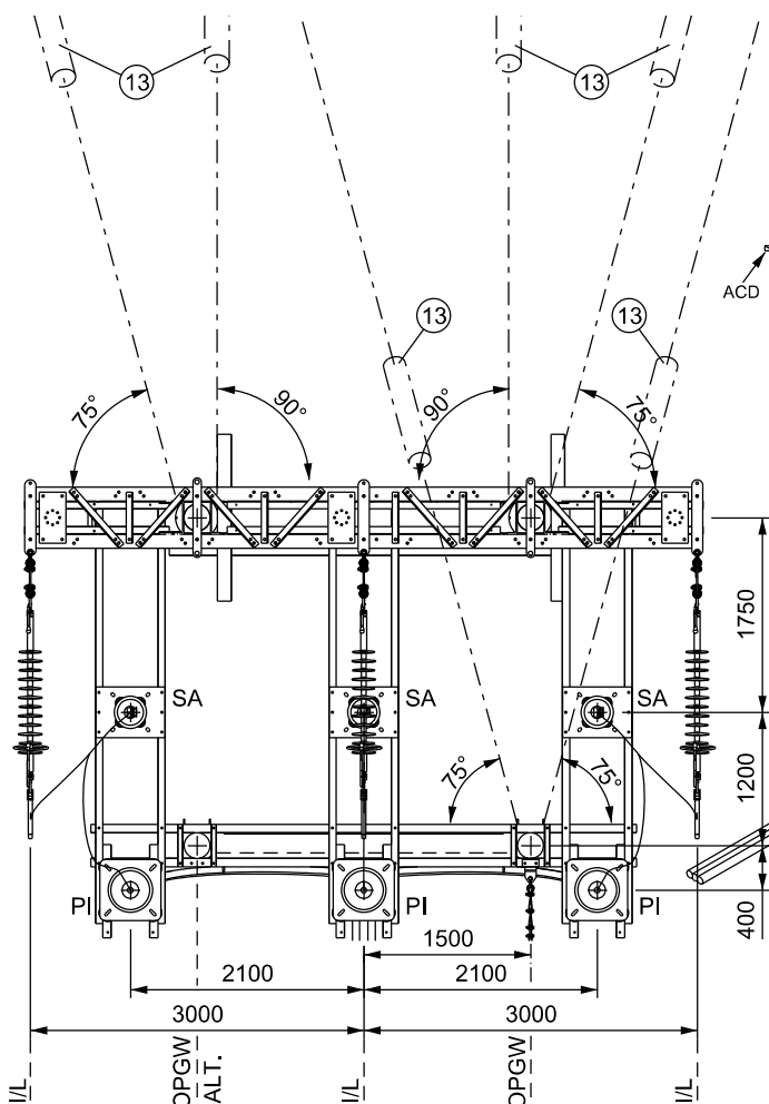
PLAN VIEW
